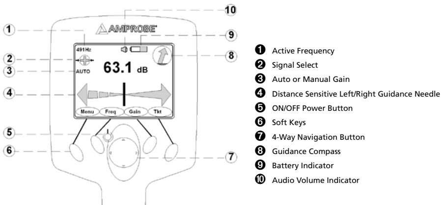
R-5000 Operational Interface
