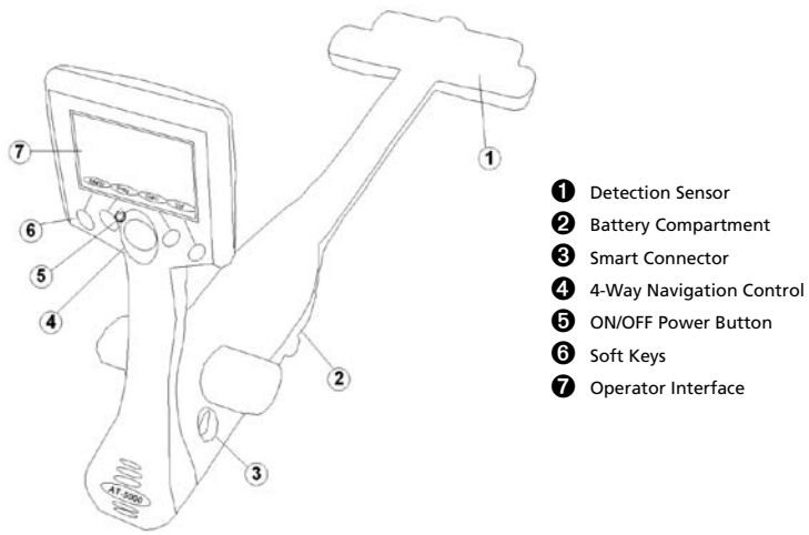
R-5000 Receiver
