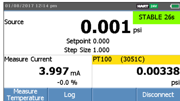
Figure 5. Triple-Function Display
