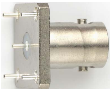
Model 7073 BNC (F) Straight PCB Mount 50 \Omega
