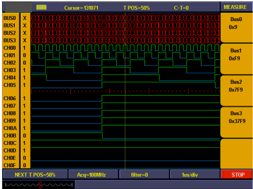
Fig 80: Bus measurement
