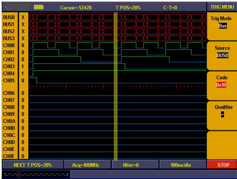
Fig 65: Bus trigger
