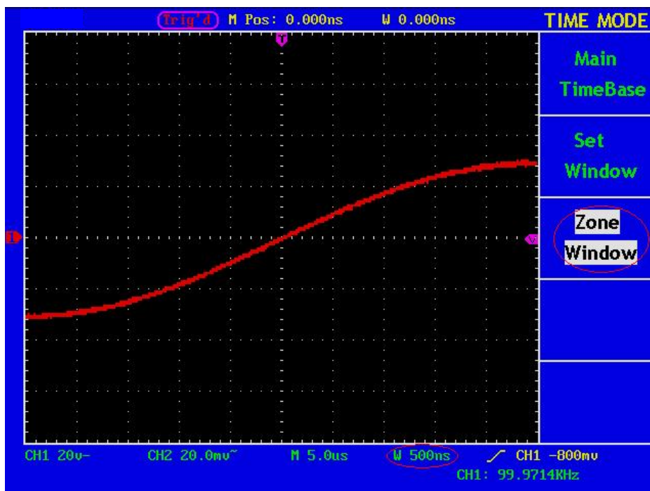
Fig. 31 Zone Window
