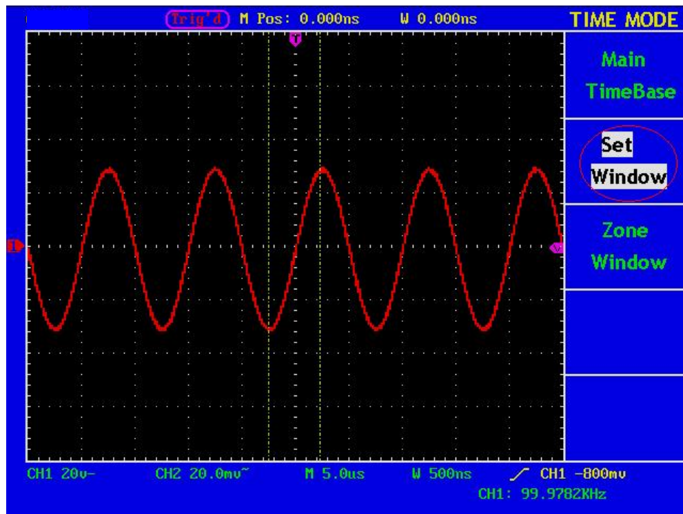
Fig. 30 Window Setting
