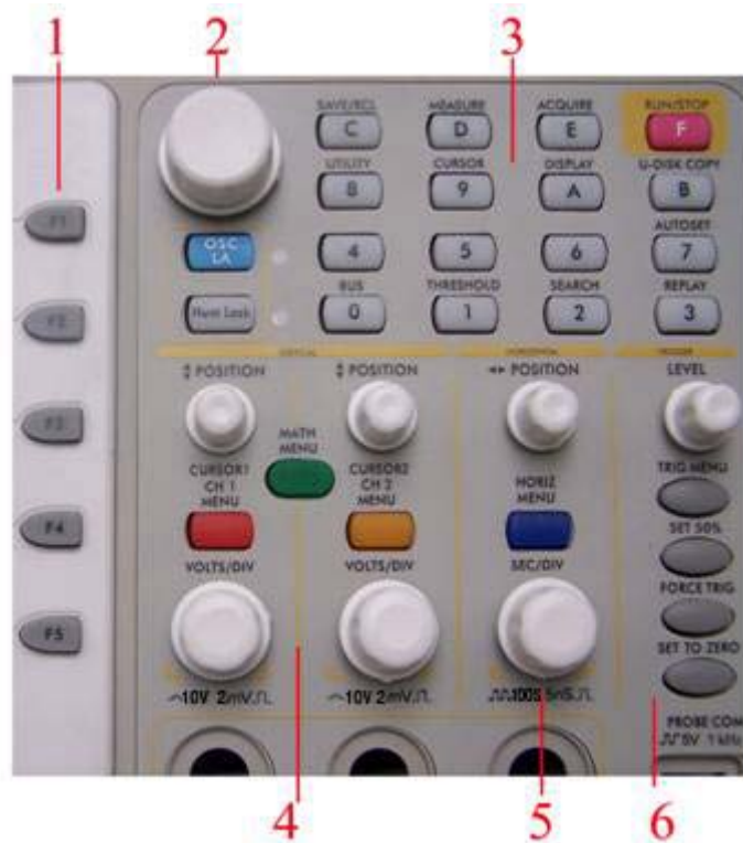
Fig 2: Keys Overview
