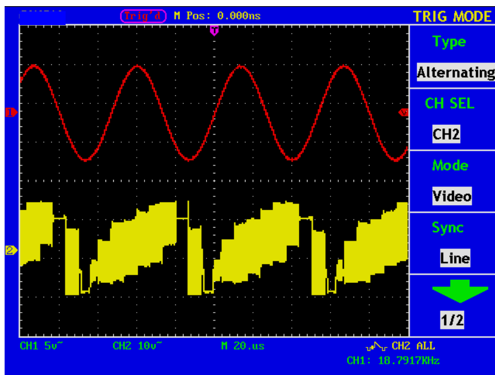
Fig. 40 Alternate trigger Oscilloscope
