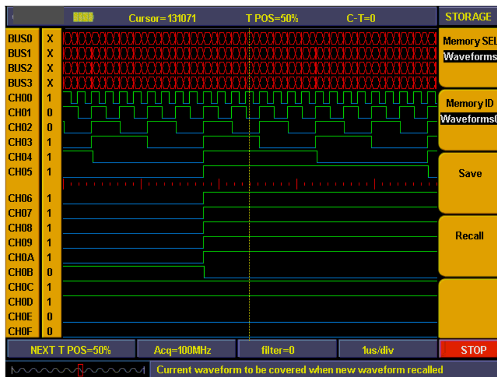
Fig 82: Waveform saving
