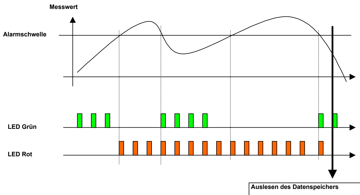
Timing Diagram: Datenlogger THC/TIC Alarme
