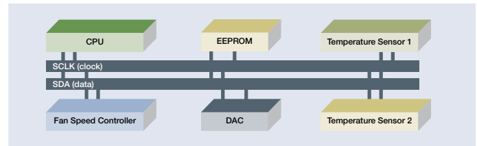
Figure 6. I 2 C bus example.
