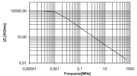
Typical input impedance PMS211A
