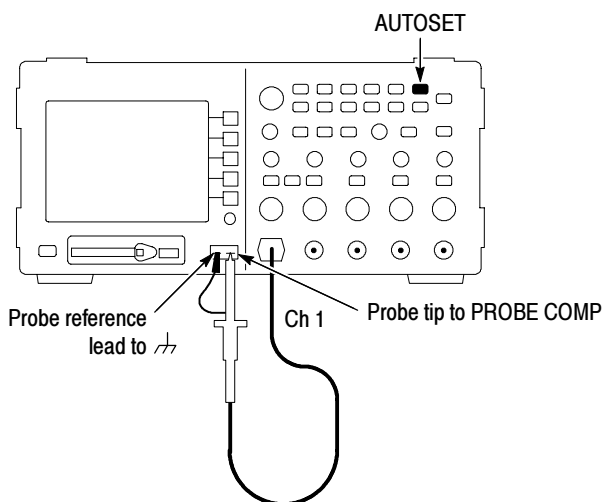
Figure 3: LF compensation setup
