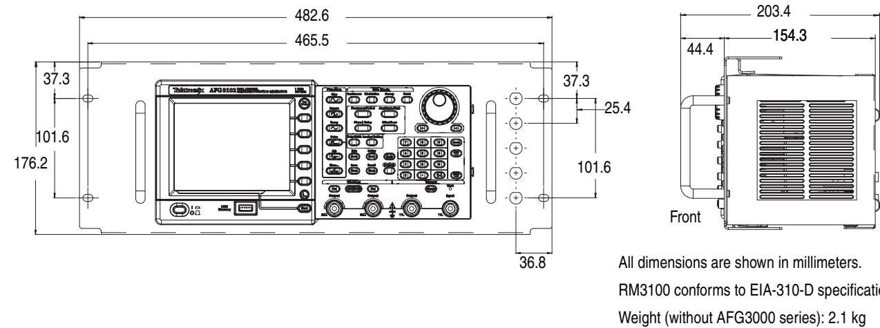
Figure 4: RM3100 Rackmount kit dimensions
