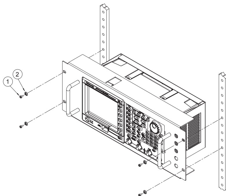
Figure 3: RM3100 Rackmount kit assembly – step 2
