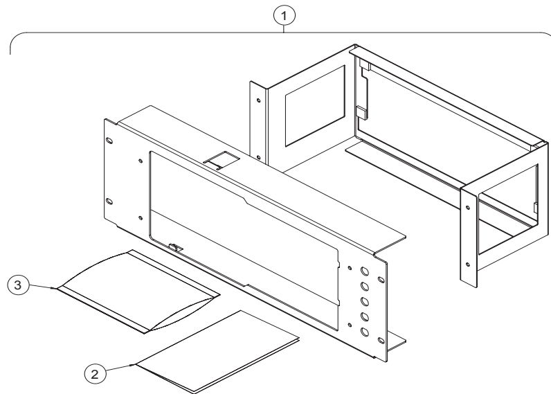
Figure 1: RM3100 Rackmount Kit
