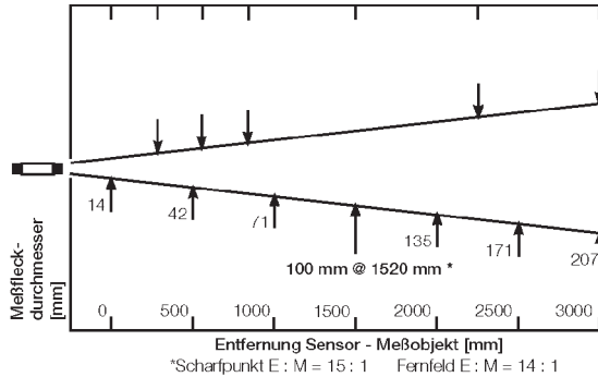
Standardoptik OS1
