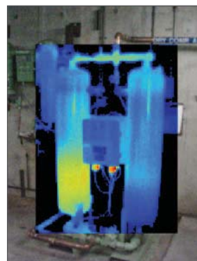
Picture-in-picture: Maintains a frame of reference by placing an IR "window" within a digital image.
