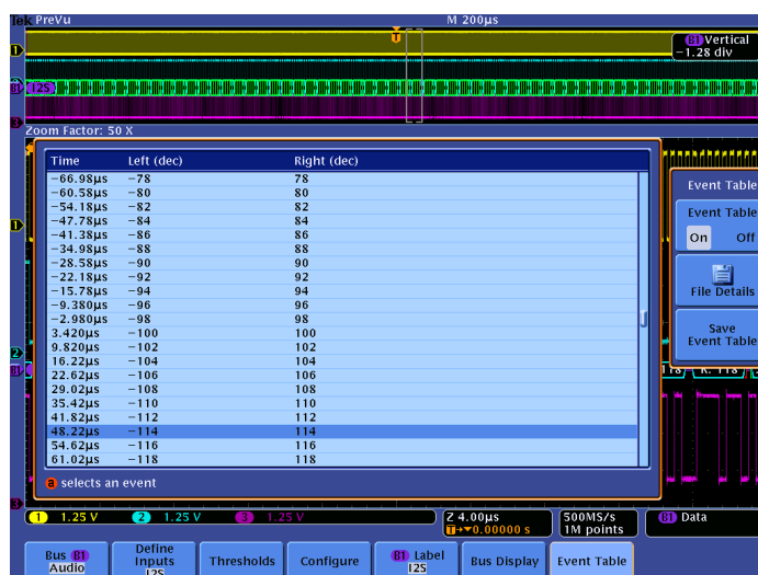
Event table for I 2 S bus with all captured packets time stamped and in a tabular view.
