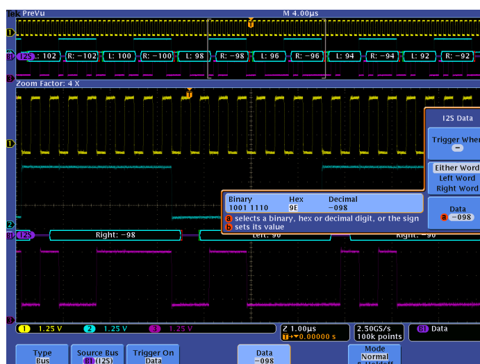
Triggering on a specific data value on the I 2 S bus.
