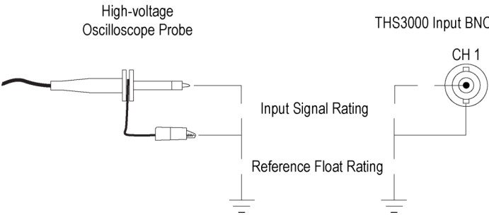
Input signal and float voltage maximum safety ratings.
